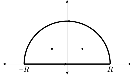
Figure 4: Contour in the upper half-plane, with the two points denoting the two simple poles of f(z) in the upper half-plane.
